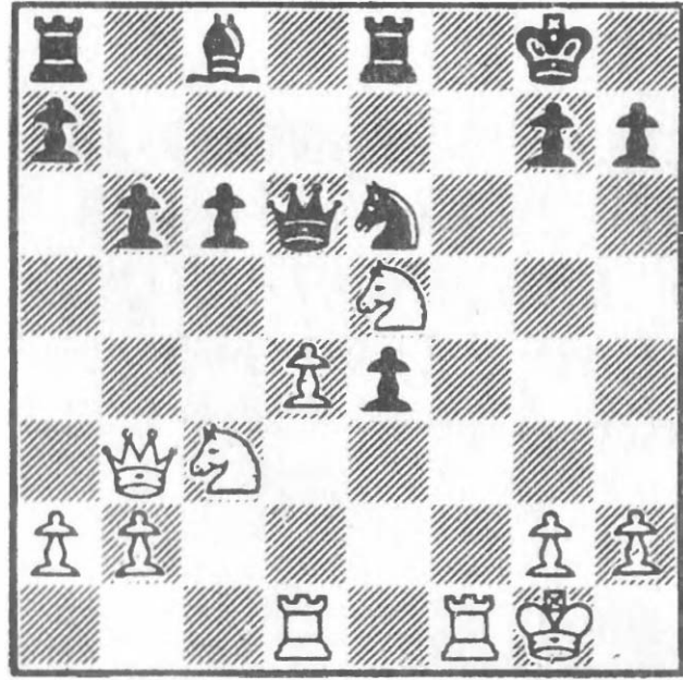
297 After 22...fxe4
